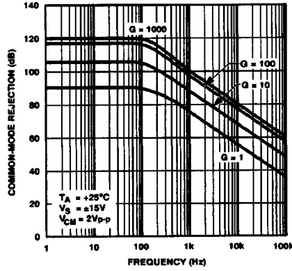
Figure 13. Common-Mode Rejection vs. Frequency
