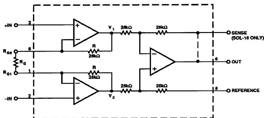
Figure 27. Triple Op Amp Topology of the AMP02
