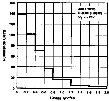
Figure 4. Typical Distribution of TCV_{IOS}
