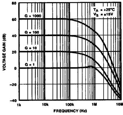
Figure 12. Closed-Loop Voltage Gain vs. Frequency
