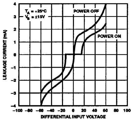
Figure 28. AMP02's Input Protection Circuitry Limits Input Current During Overvoltage Conditions
