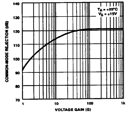
Figure 14. Common-Mode Rejection vs. Voltage Gain
