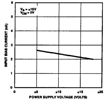
Figure 11. Input Bias Current vs. Supply Voltage
