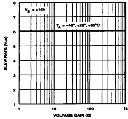
Figure 25. Slew Rate vs. Voltage Gain
