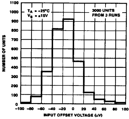
Figure 3. Typical Distribution of Input Offset Voltage
