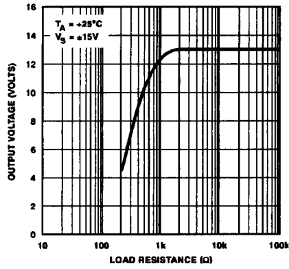
Figure 22. Maximum Output Voltage vs. Load Resistance
