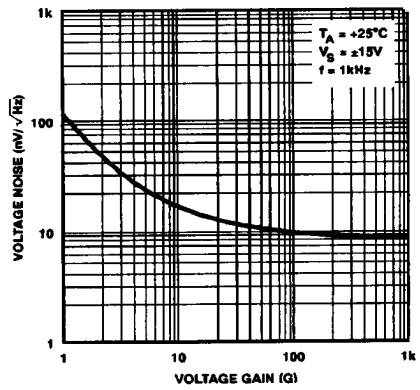
Figure 19. RTI Voltage Noise Density vs. Gain
