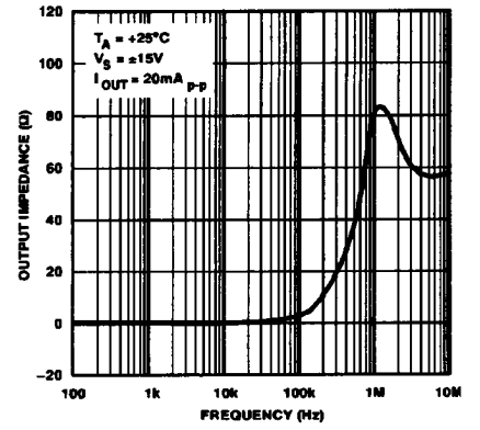
Figure 23. Closed Loop Output Impedance vs. Frequency
