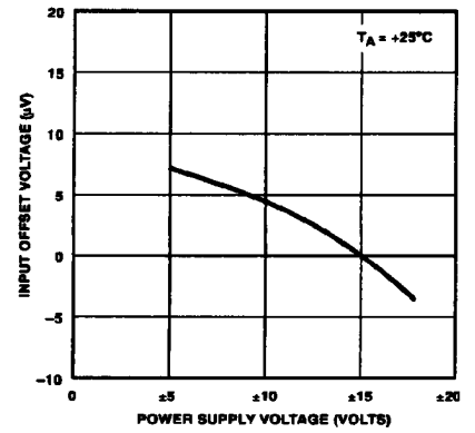
Figure 5. Input Offset Voltage Change vs. Supply Voltage
