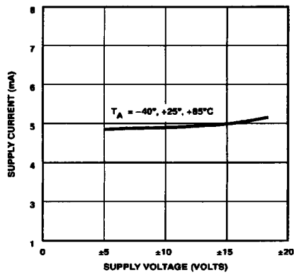
Figure 24. Supply Current vs. Supply Voltage
