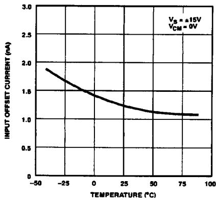
Figure 9. Input Offset Current vs. Temperature
