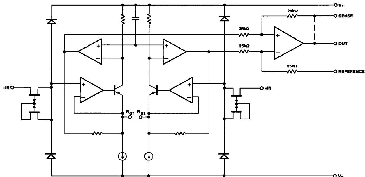
Figure 2. Simplified Schematic
