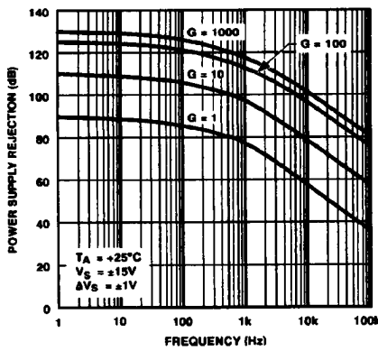
Figure 15. Positive PSR vs. Frequency
