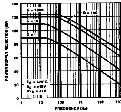
Figure 16. Negative PSR vs. Frequency
