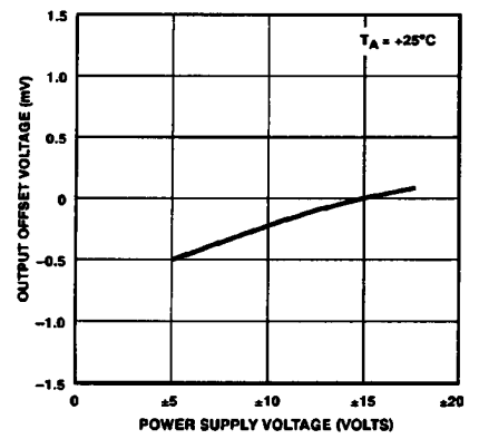
Figure 8. Output Offset Voltage Change vs. Supply Voltage
