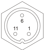
Switchcraft EN3 Panel Connector (Front View)
