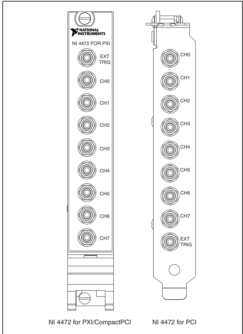
Figure 2-1. NI 4472 Front Panels
